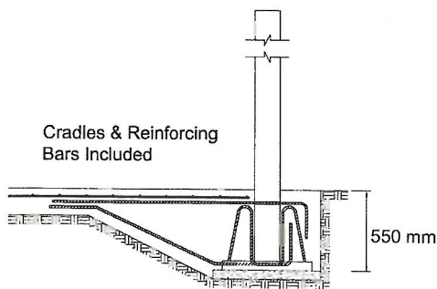
Typical Foundation Detail
