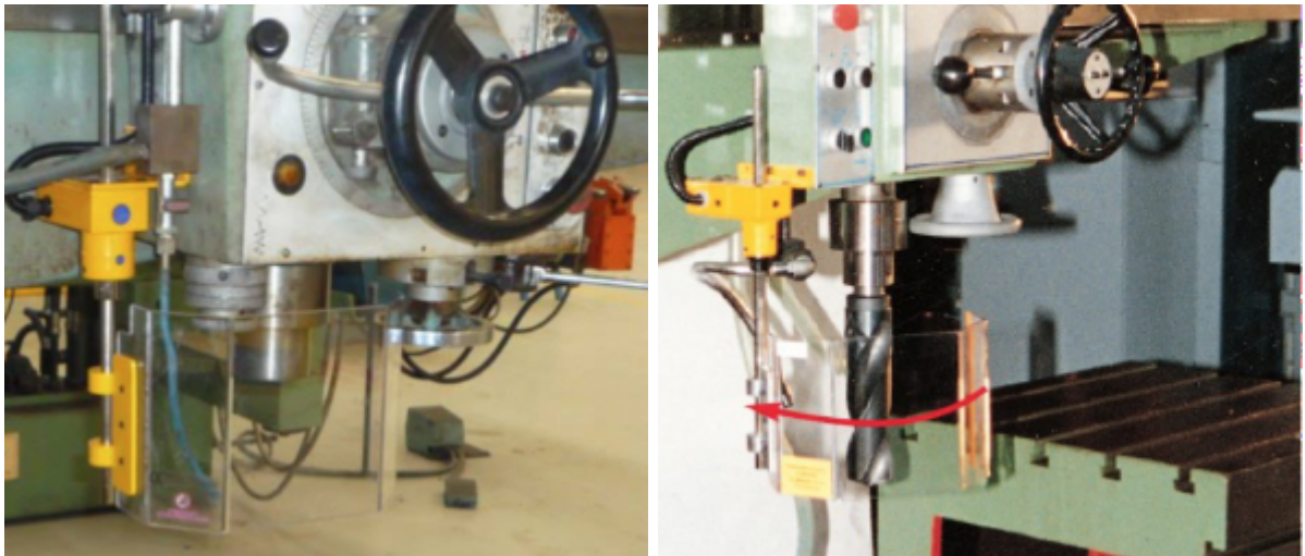
10. TR3A (300mm wide x 200mm high) This is ideal for radial drilling machines.
