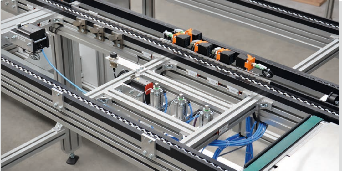
Versamove plus: Customer-specific special stopper unit with four removal positions
