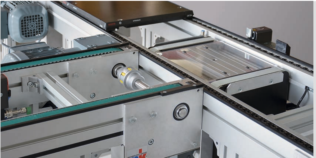
Versamove standard: Lift and transfer with damped stop
