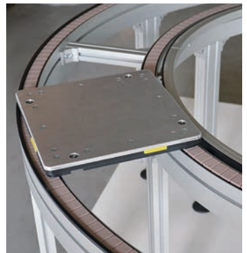
Versamove standard: Flat top chain conveyor curve
