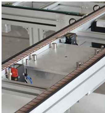
Versamove standard: Stopper and lift and locate
