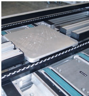
Versamove plus: Dual-lane system with special guide rails
