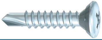
Countersunk (Ribbed) Self Drill PVC Screw
