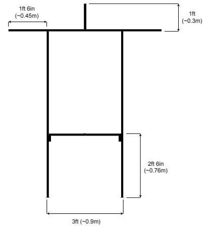
ASSEMBLY
