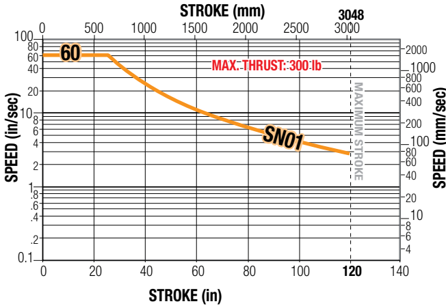
Critical Speed: 0.75" 1TPI Acme Screw
