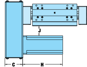
REVERSE-PARALLEL RIGHT (RPR) mounting surface shown UP
