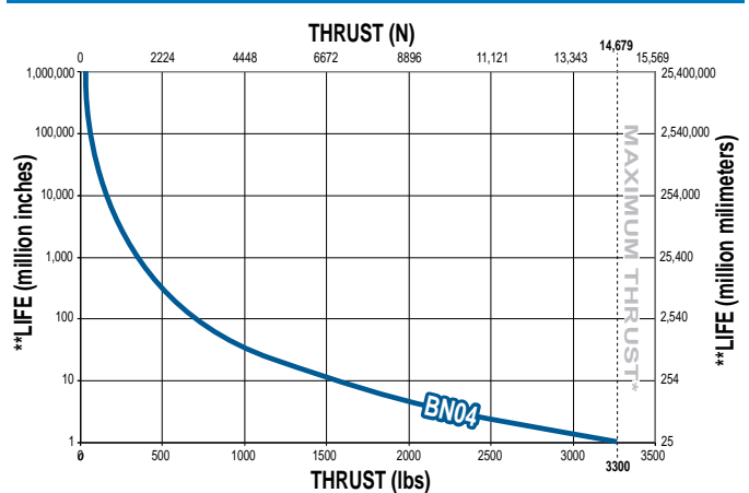
Life: 1", 4TPI Ball Screw
