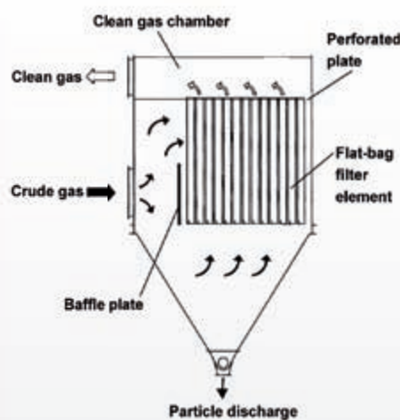
Crude gas inlet from above and below The partial inlet from below hinders the falling down of particularly the fine particles into the collection hopper.
