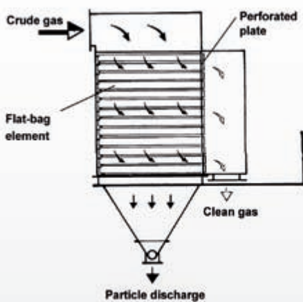
Crude gas inlet 100 % from above Downstream principle favours the falling down of particles into the collection hopper.
