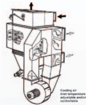
Flat-tube heat exchanger with cooling air recirculation
