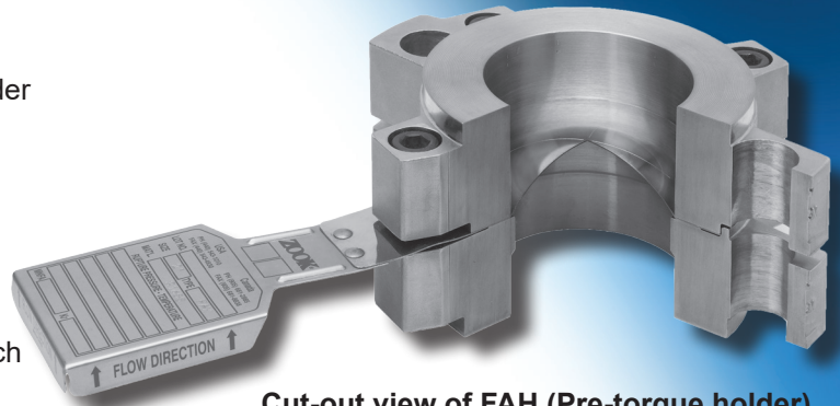
Cut-out view of FAH (Pre-torque holder)
