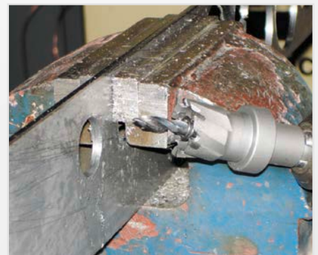
Free-hand drilling up to Ø 30 mm
