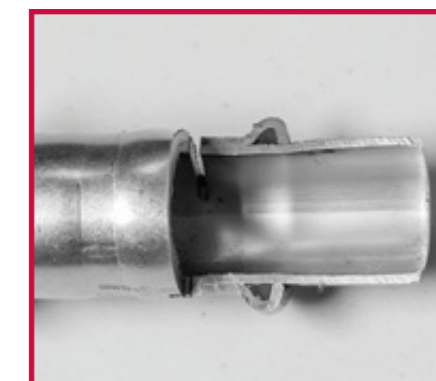
6. Correctly pressed fitting.
