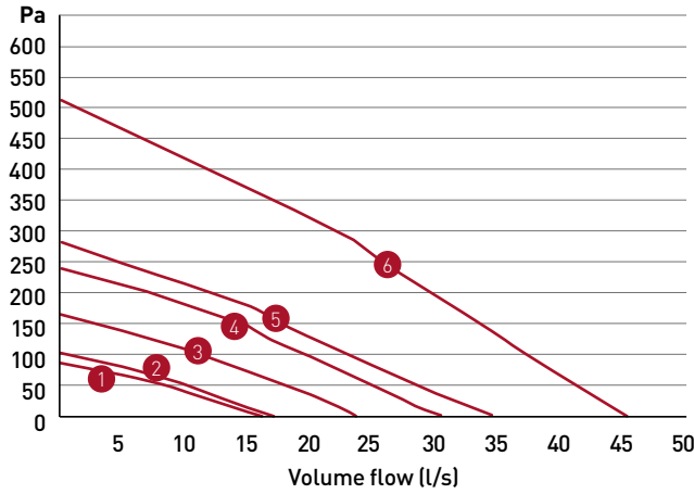
AQH200-S
