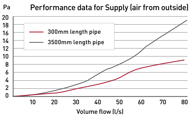
204x60 – Ø150mm
