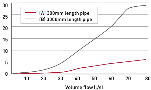
Pa Performance data for Supply (air from outside)
