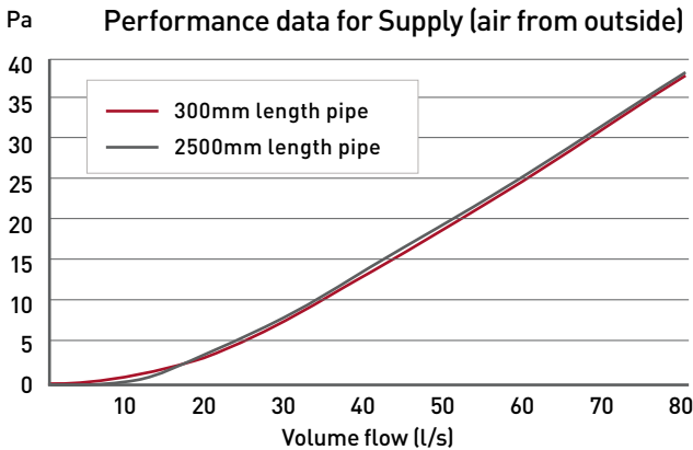
204x60 – Ø125mm
