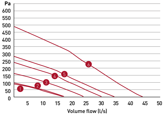
AQH200-B
