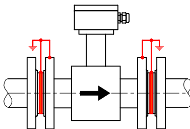
Fig.16: Grounding rings
