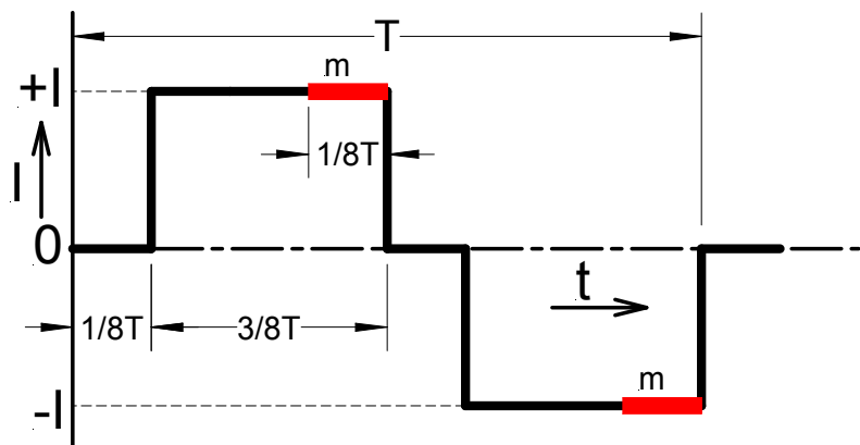
Fig. 2 - Excitation pulse form
