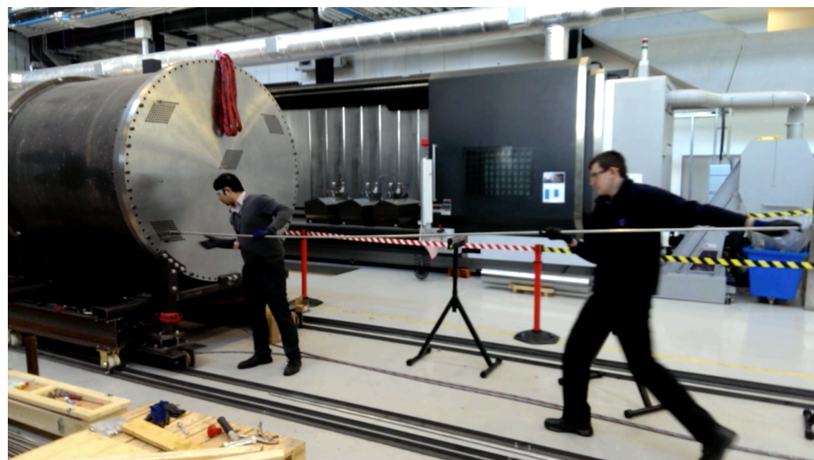
Sizewell C primary heat exchangers under assembly test
