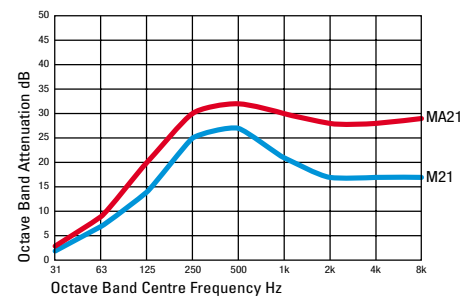
6" Bore
