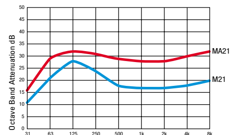
24" Bore
