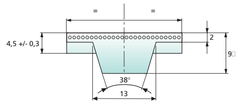
notched guide
