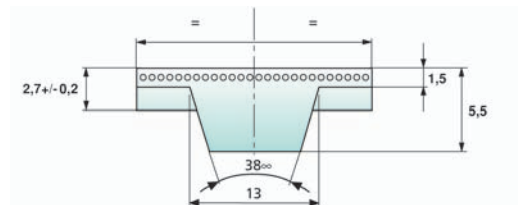
notched guide
