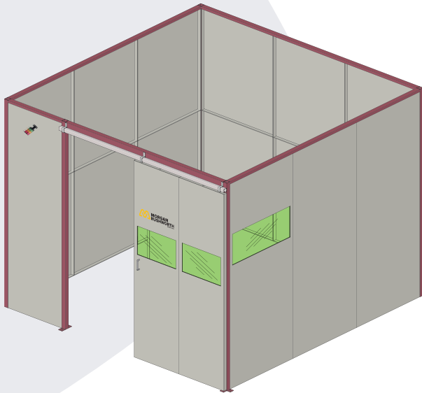
An example of a 3m x 3m enclosure with a sliding door instead of hinged
